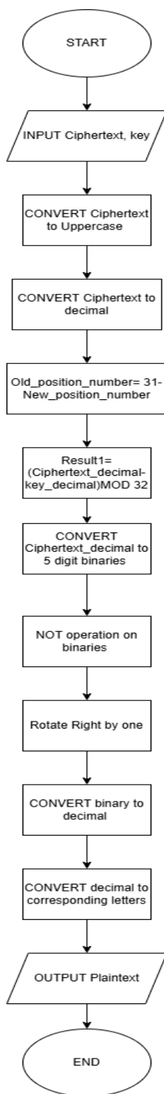
Figure 11: Decryption Flowchart
